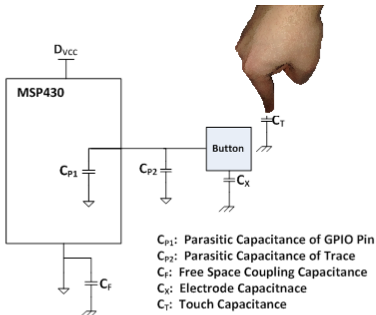
Figure 1. Capacitive Circuit Model – MCU Independent
