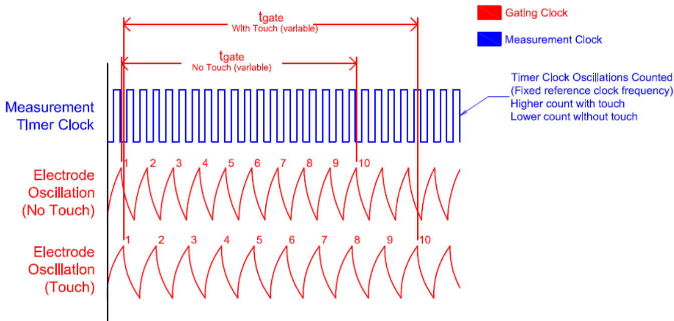
Figure 5. fRO Measurement Timing Diagram
